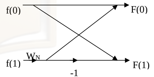
Fig(c): FFT Butterfly for 2-point DFT.
